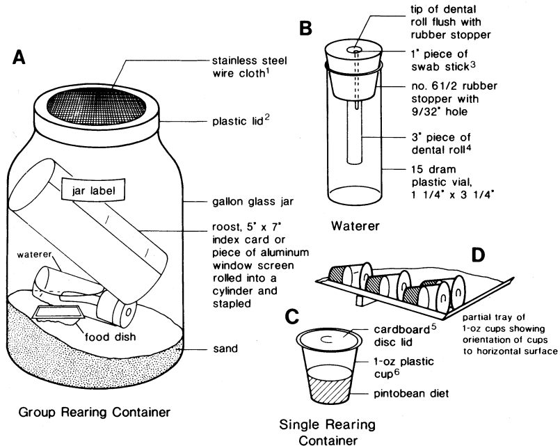
Fig. 1. A. Group rearing container. B. Waterer. C. Single rearing container. D. Holding tray. (1" = 2.54 cm) Notes (referenced by superscript numbers): (1) Stainless steel wire cloth, 60 mesh/inch, .0075" dia wire, .0092" width of opening, 30.5% open area. McNichols Co., 5501 Gray St., Tampa, FL 33609. [Wire window screen can be substituted, but it will admit ants and small spiders.] (2) 3/4" O.D. plastic lid, Dynalab Corp., P.O. Box 112, Rochester, NY 14692. (3) Piece of swab stick prevents vacuum from forming and causing the exposed tip of dental roll to become dry. (4) No. 2 (3/8" dia), 6-inch dental roll. Johnson and Johnson, New Brunswick, NJ 08903. Hand-rolled cotton or cloth might work. (5) Cardboard disc lid, 1.476" dia, no wax, no staples, pull tab. Standard Cap and Seal Co., P.O. Box 1766, Norton, GA 30091. (6) #410 clear plastic cup. Fill-Rite Inc., 49-55 Liberty St., Newark, NJ 07102.
